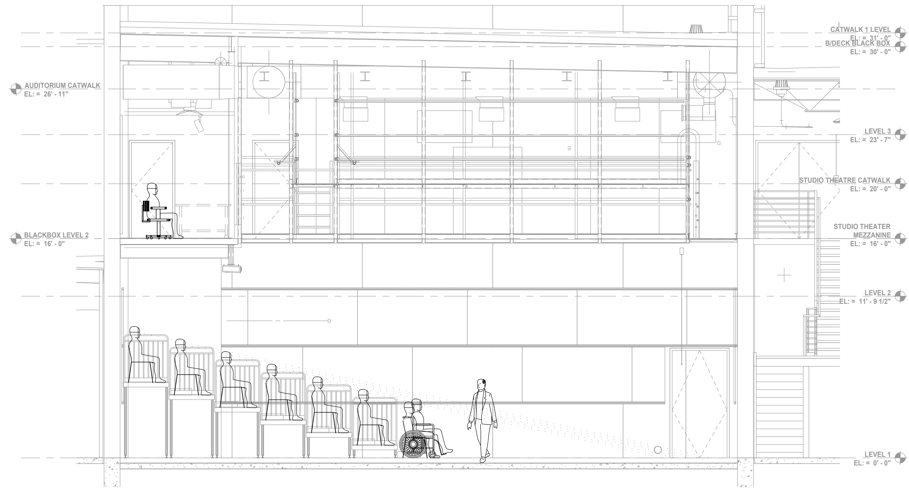
13 SECTION - END STAGE SEATING LAYOUT B SCALE: 1/4" = 1'-0"
