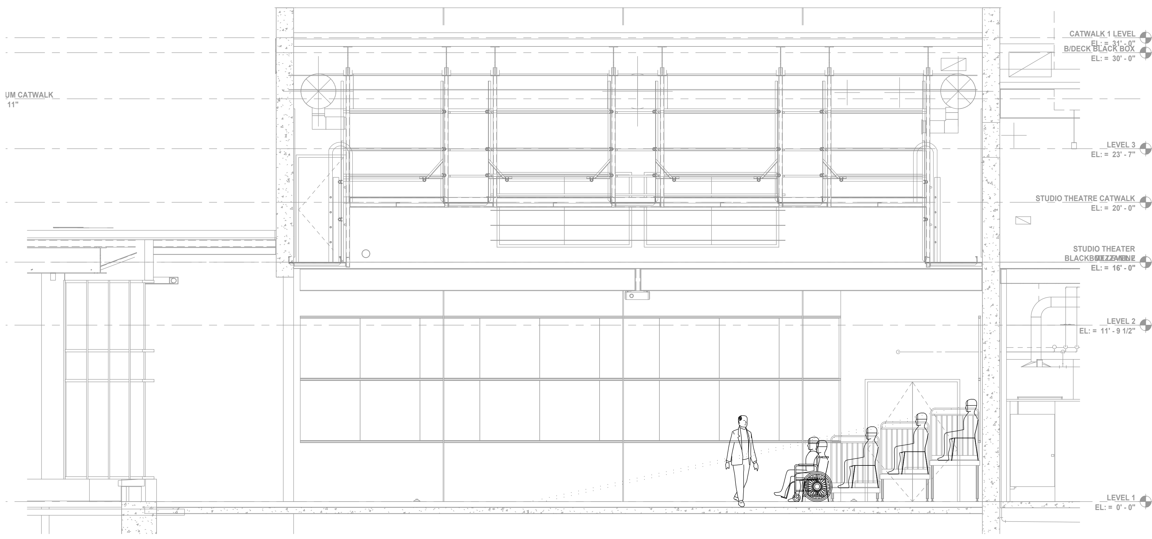
3 SECTION - THRUST SEATING LAYOUT A SCALE: 1/4" = 1'-0"
