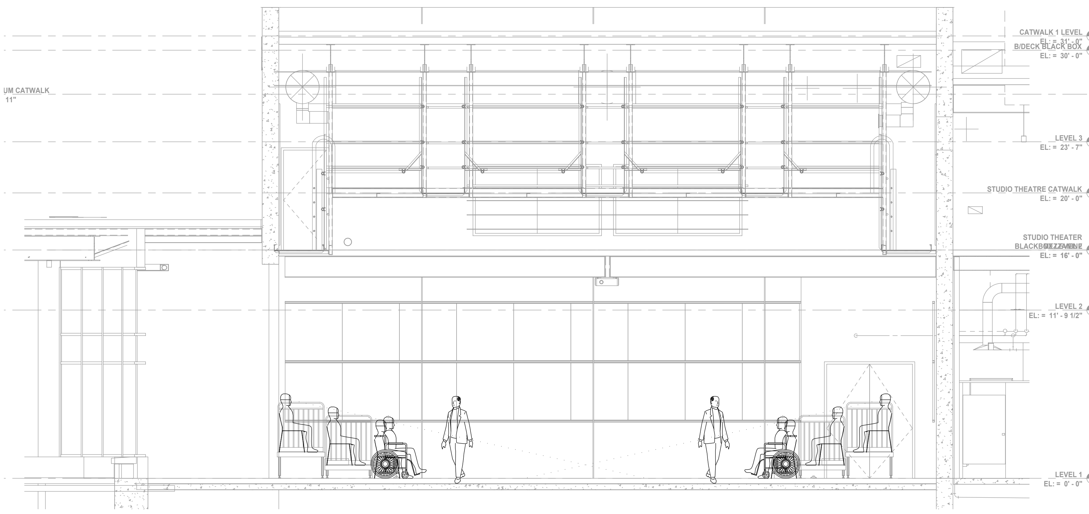
13 SECTION - THRUST SEATING LAYOUT B SCALE: 1/4" = 1'-0"
