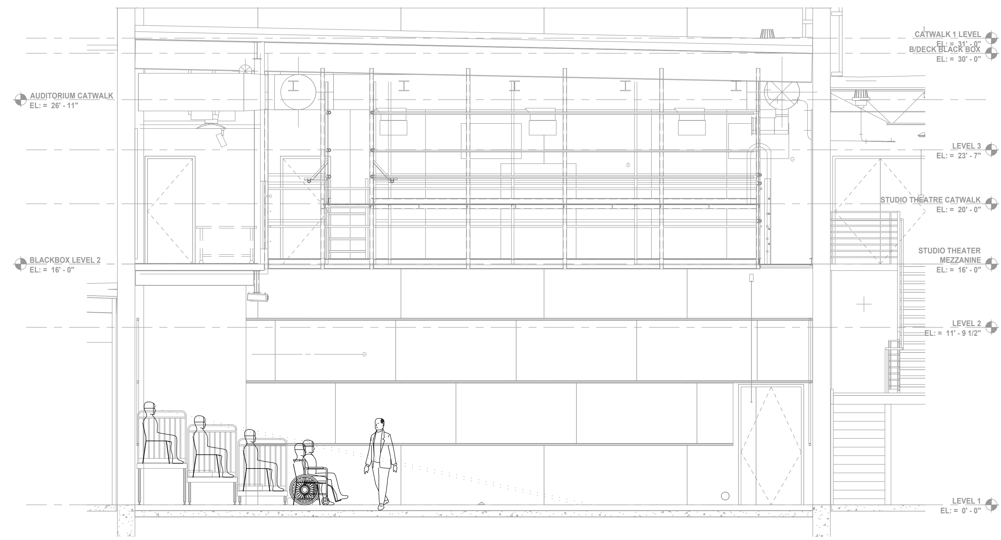
14 SECTION - CORNER SEATING LAYOUT SCALE: 1/4" = 1'-0"
