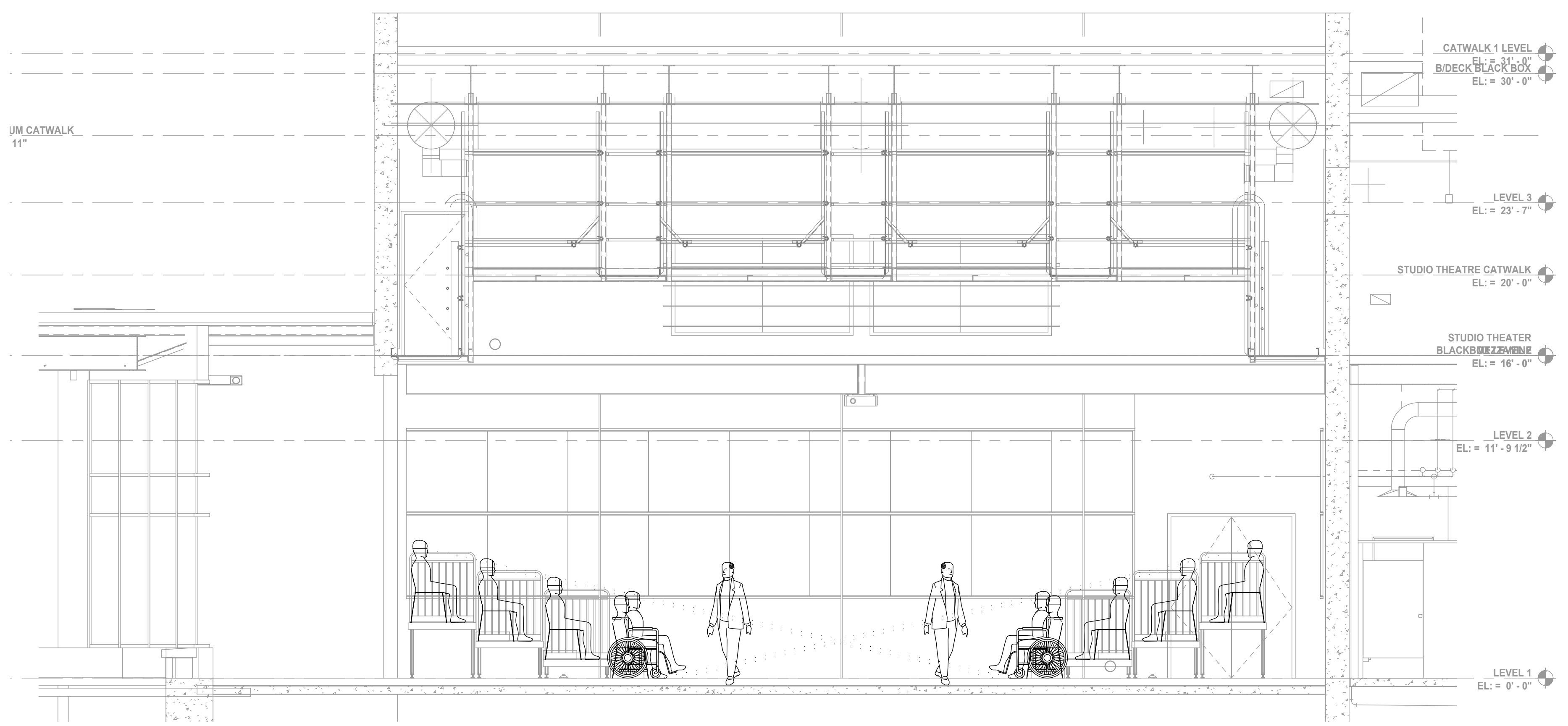
13 SECTION - PROMENADE SEATING LAYOUT A SCALE: 1/4" = 1'-0"
