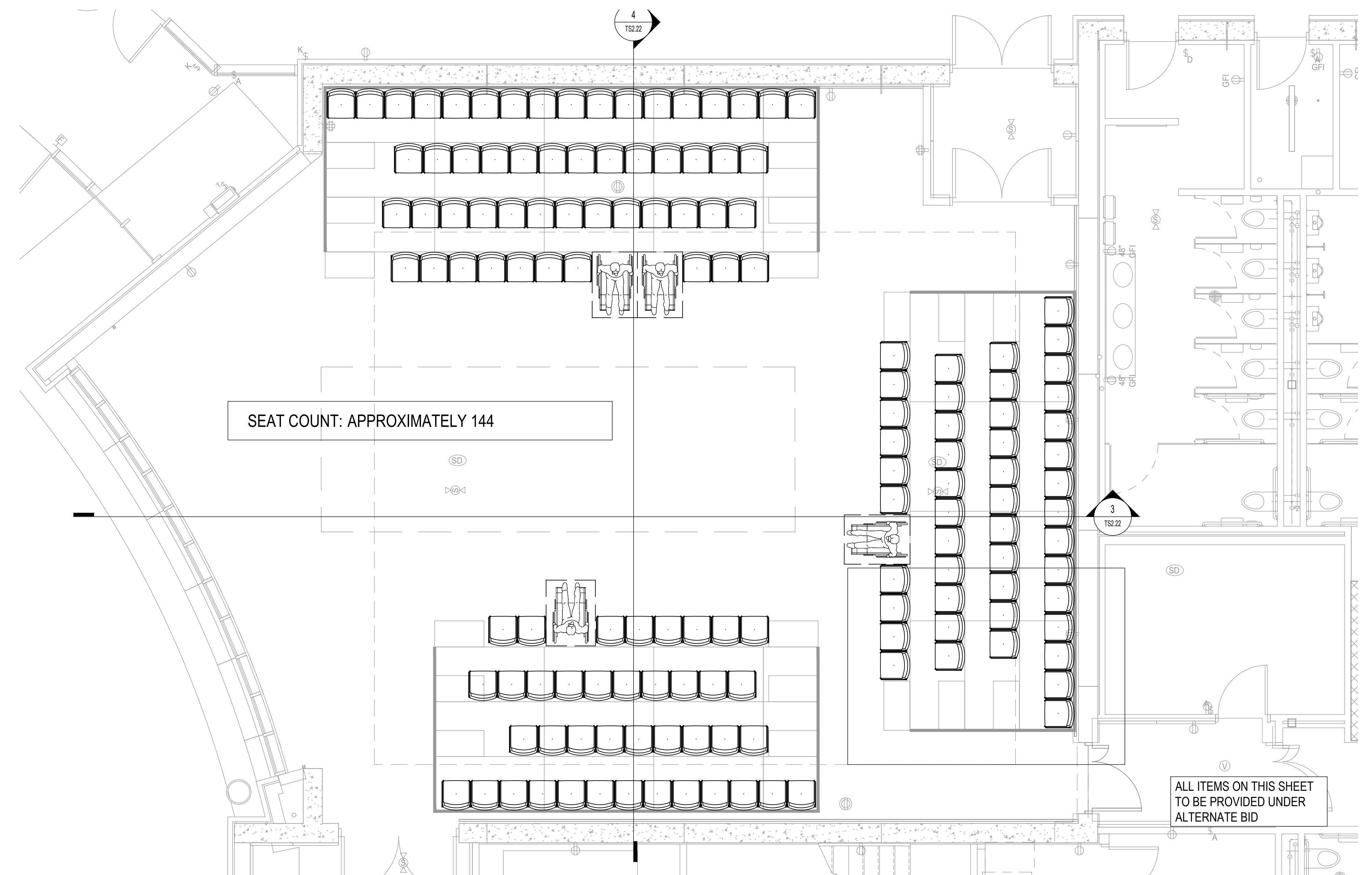
3 PLAN - THRUST SEATING LAYOUT A SCALE: 1/4" = 1'-0"
