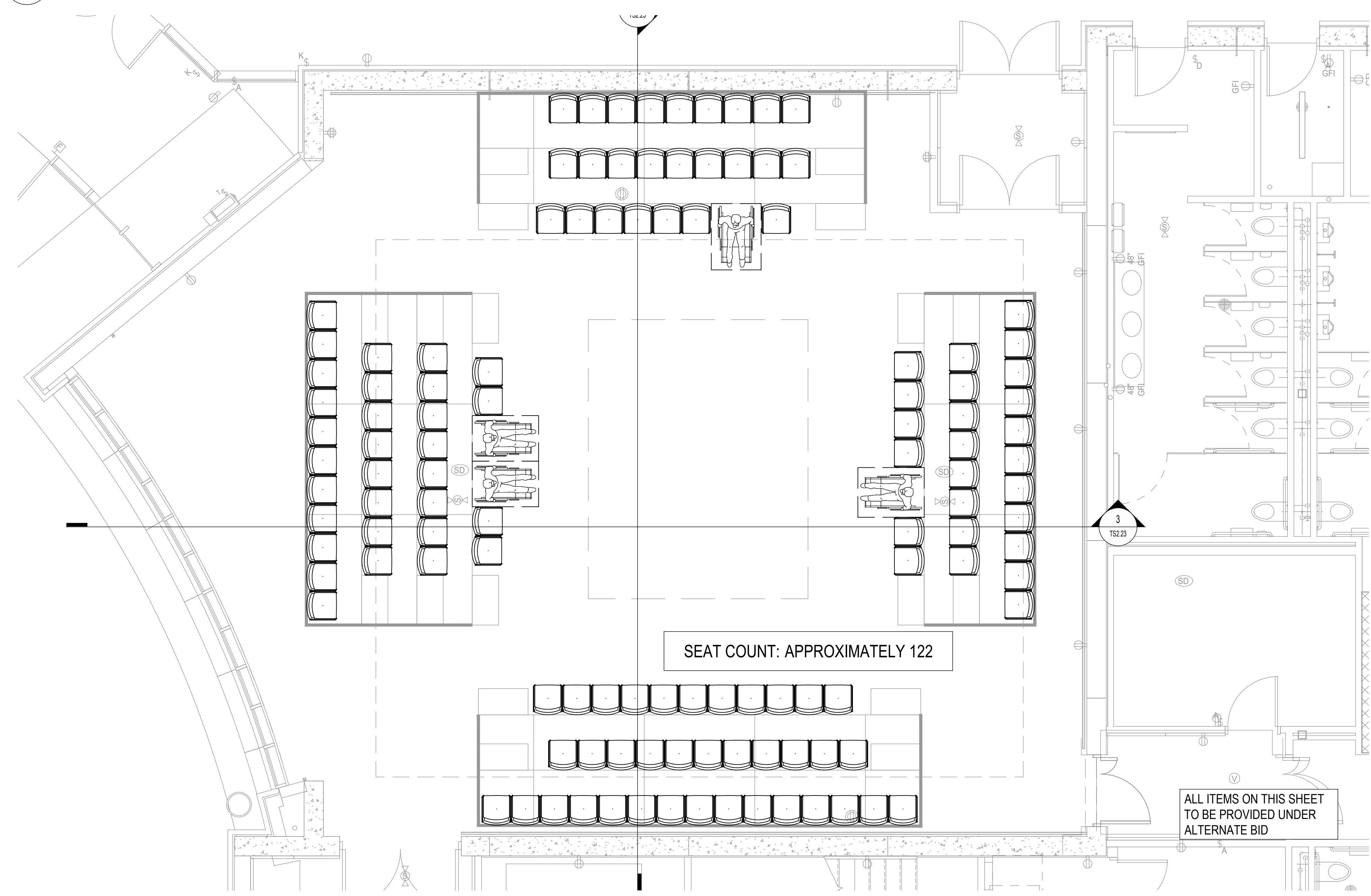
3 PLAN - ARENA SEATING LAYOUT SCALE: 1/4" = 1'-0"
