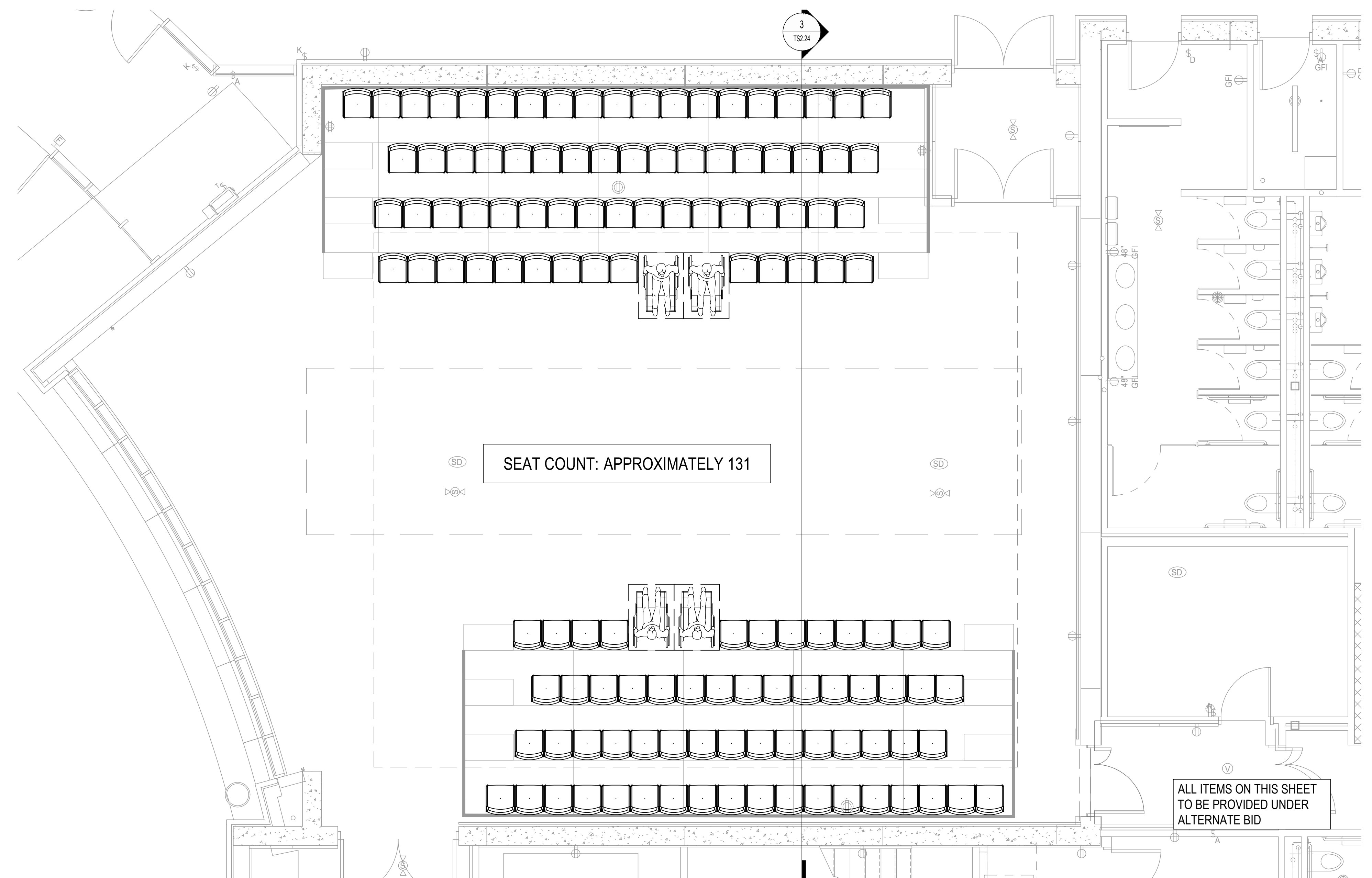
3 PLAN - PROMENADE SEATING LAYOUT B SCALE: 1/4" = 1'-0"
