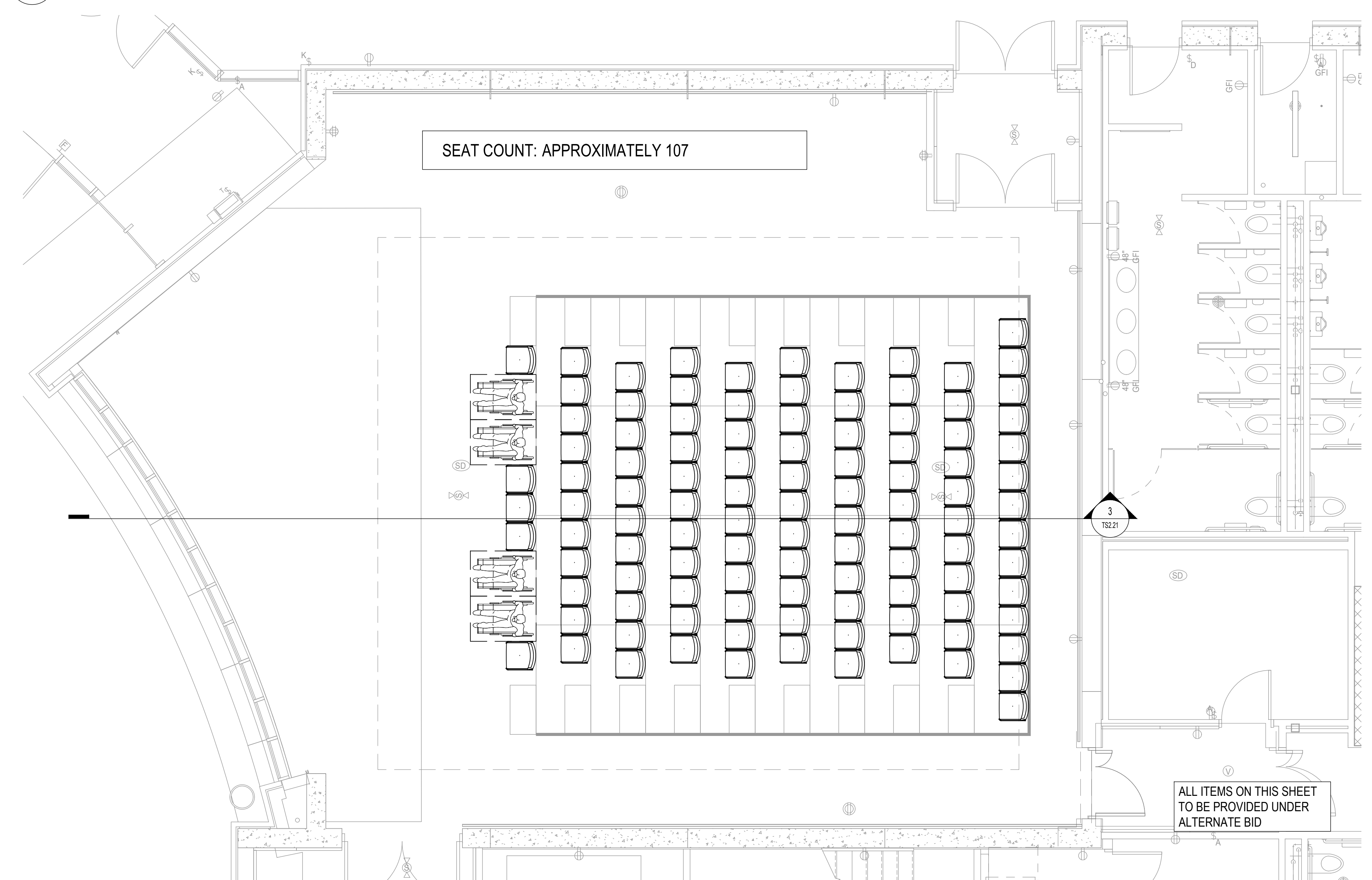
3 PLAN - END STAGE SEATING LAYOUT A SCALE: 1/4" = 1'-0"
