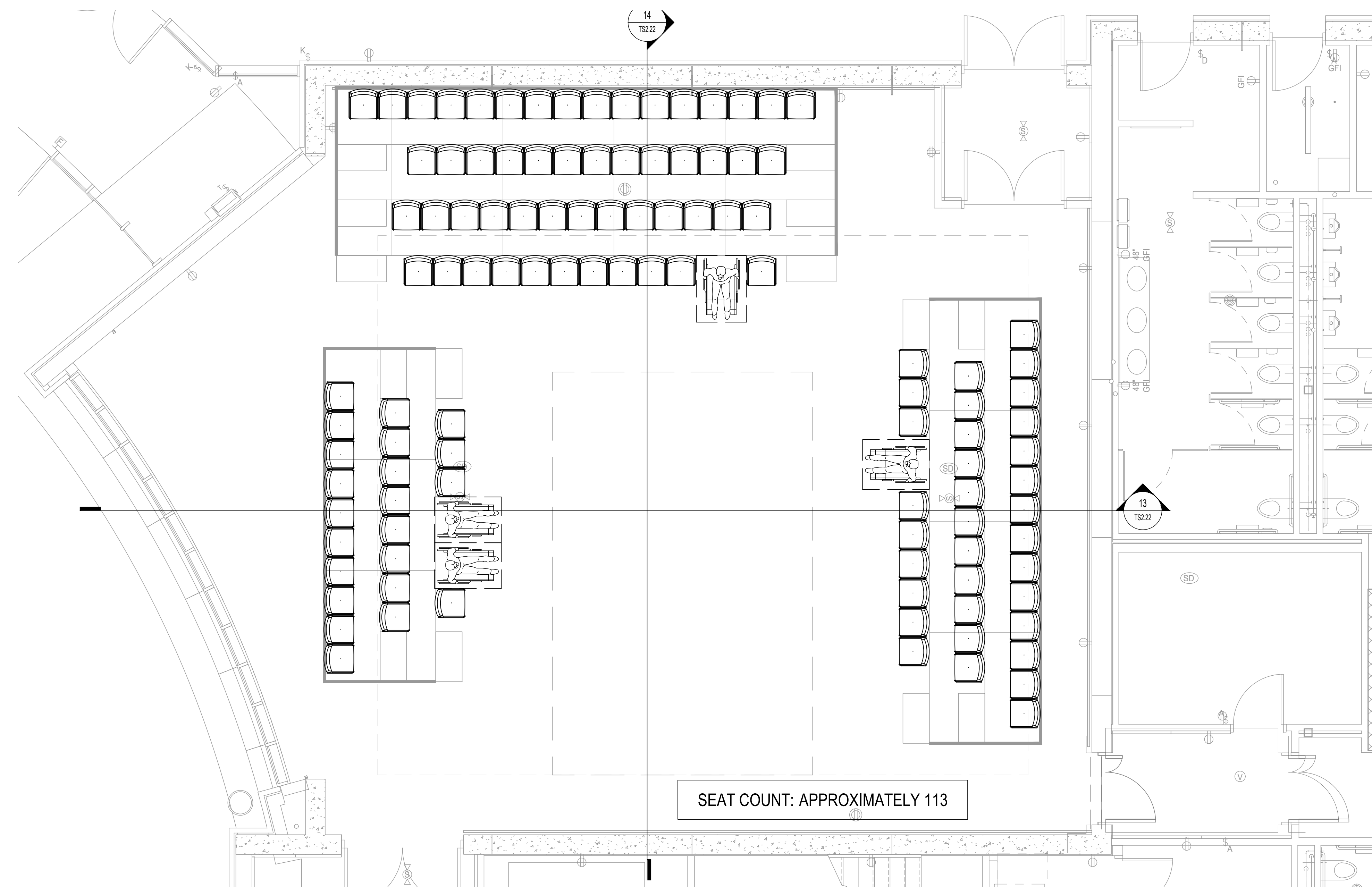
11 PLAN - THRUST SEATING LAYOUT B SCALE: 1/4" = 1'-0"
