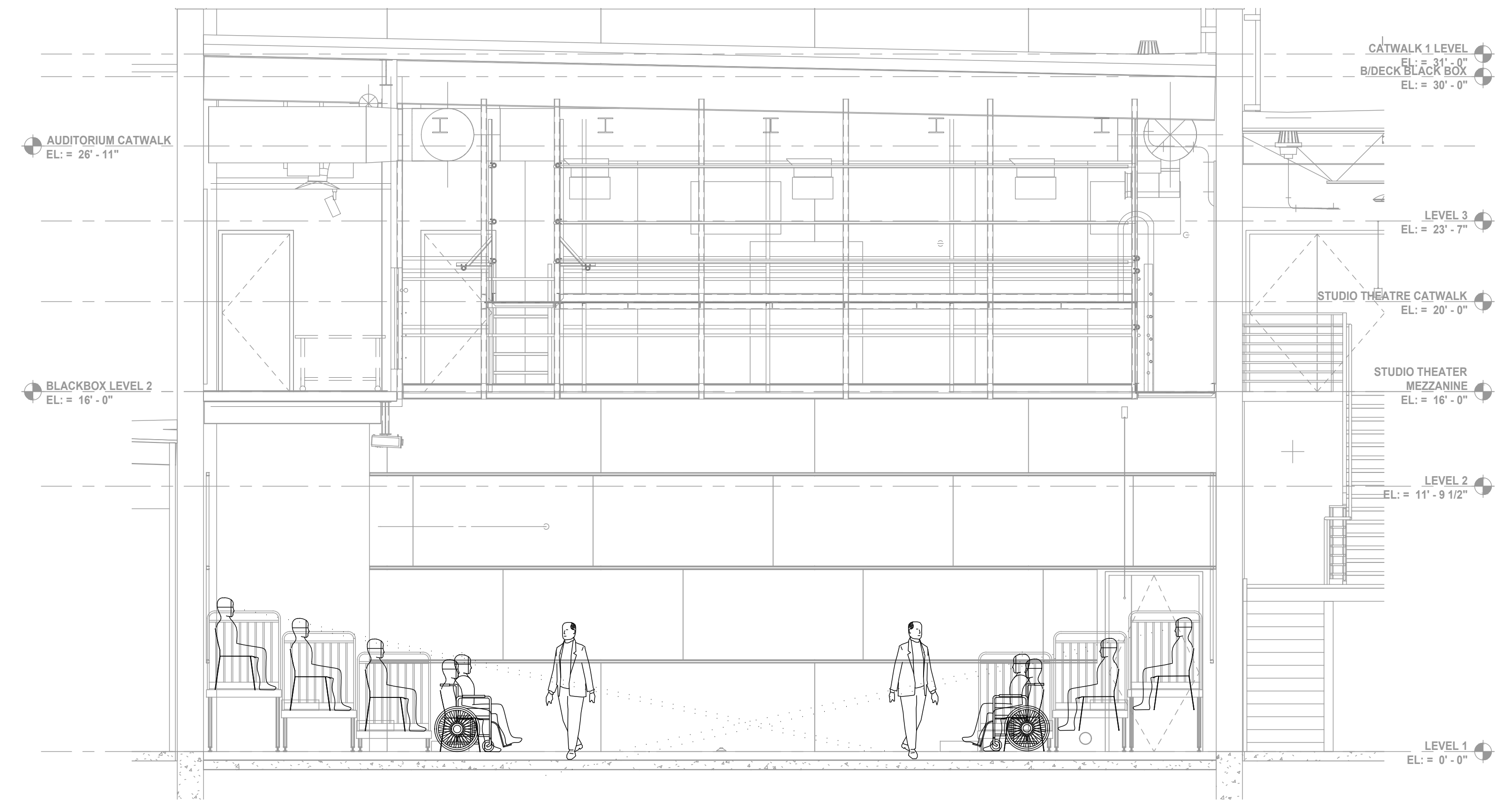
3 SECTION - PROMENADE SEATING LAYOUT B SCALE: 1/4" = 1'-0"
