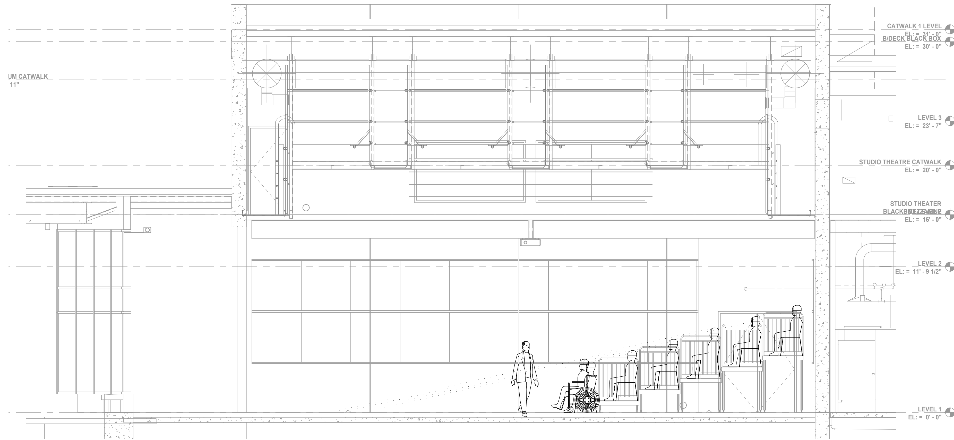
13 SECTION - CORNER SEATING LAYOUT SCALE: 1/4" = 1'-0"
