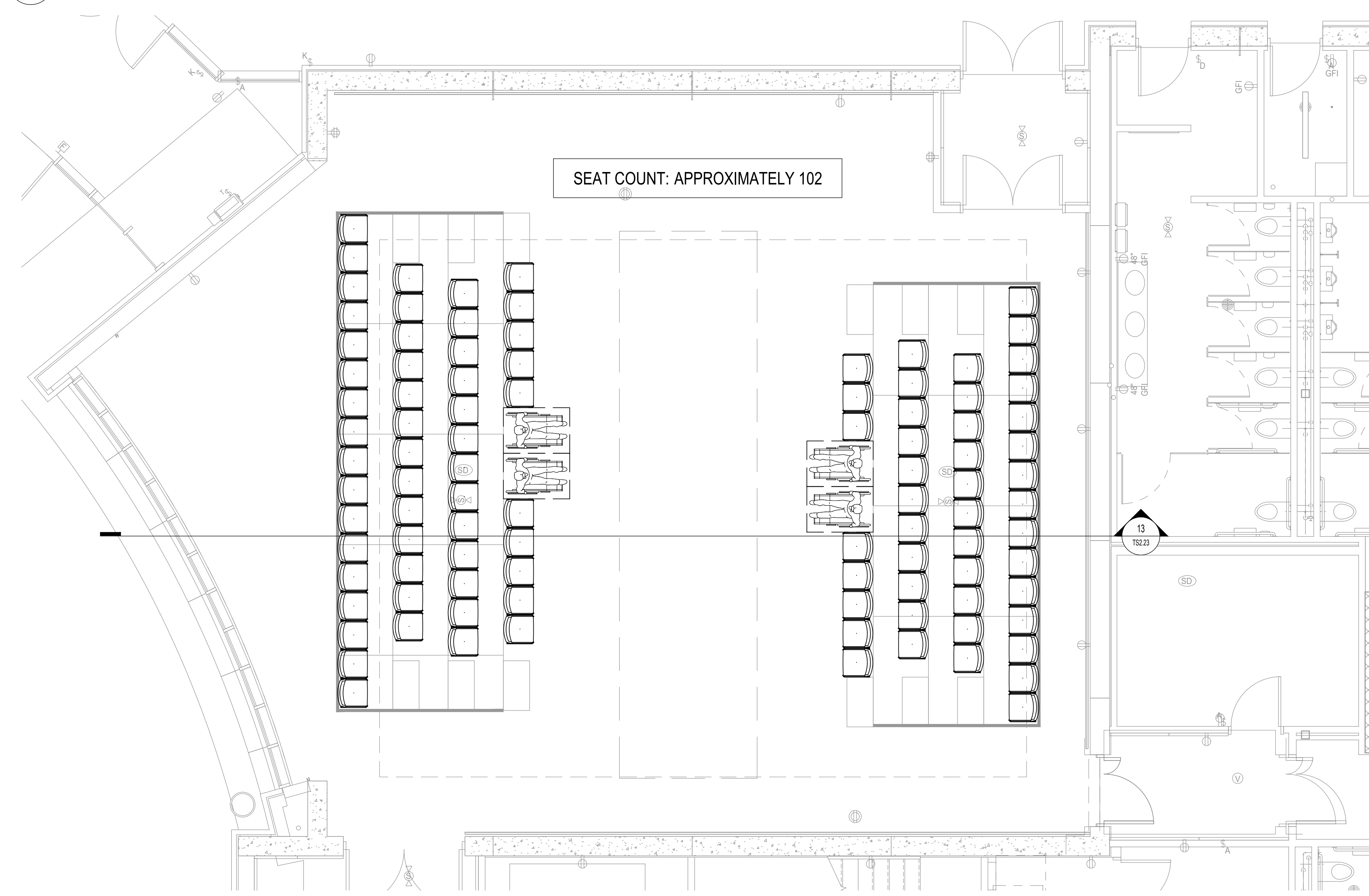
11 PLAN - PROMENADE SEATING LAYOUT A SCALE: 1/4" = 1'-0"
