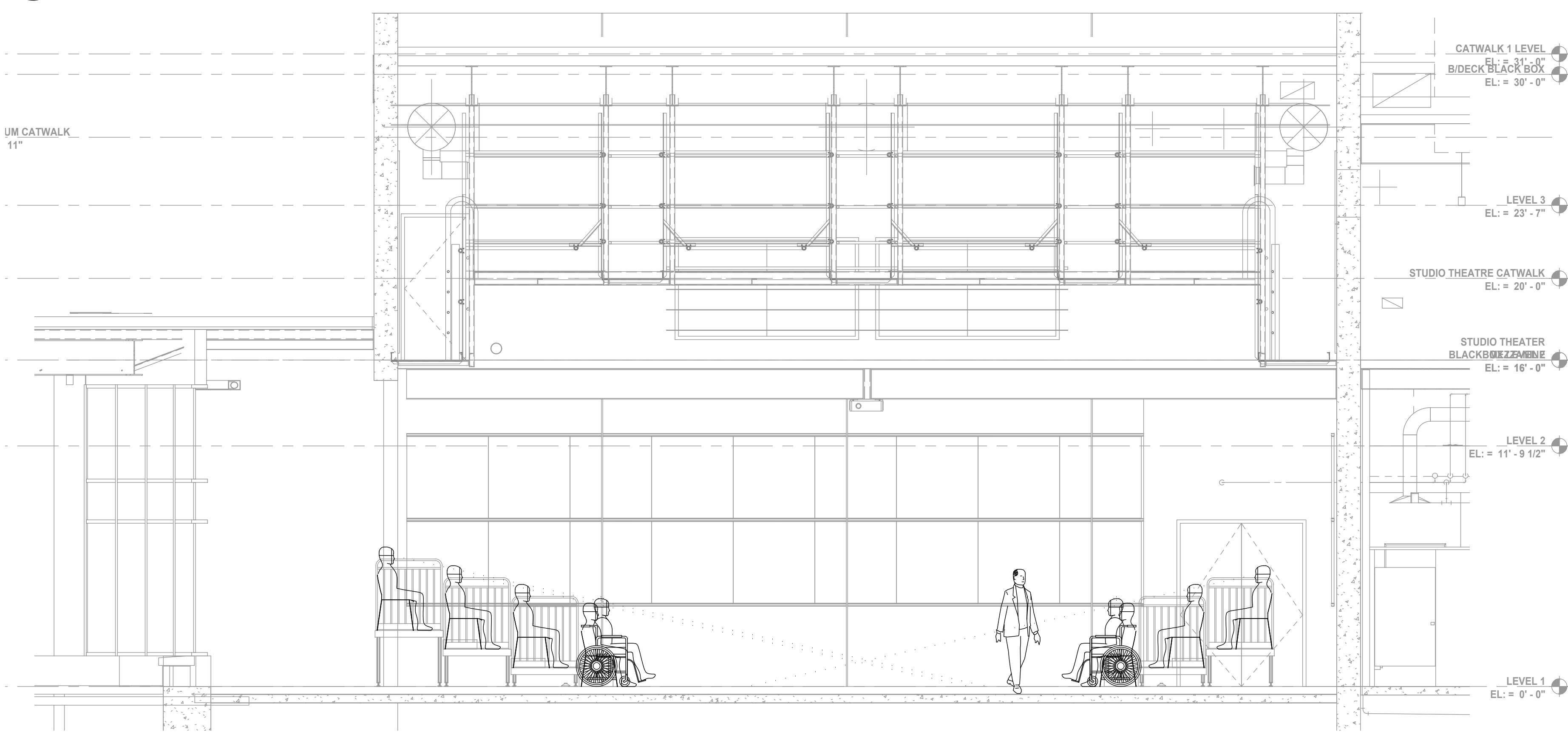
3 SECTION - ARENA SEATING LAYOUT SCALE: 1/4" = 1'-0"
