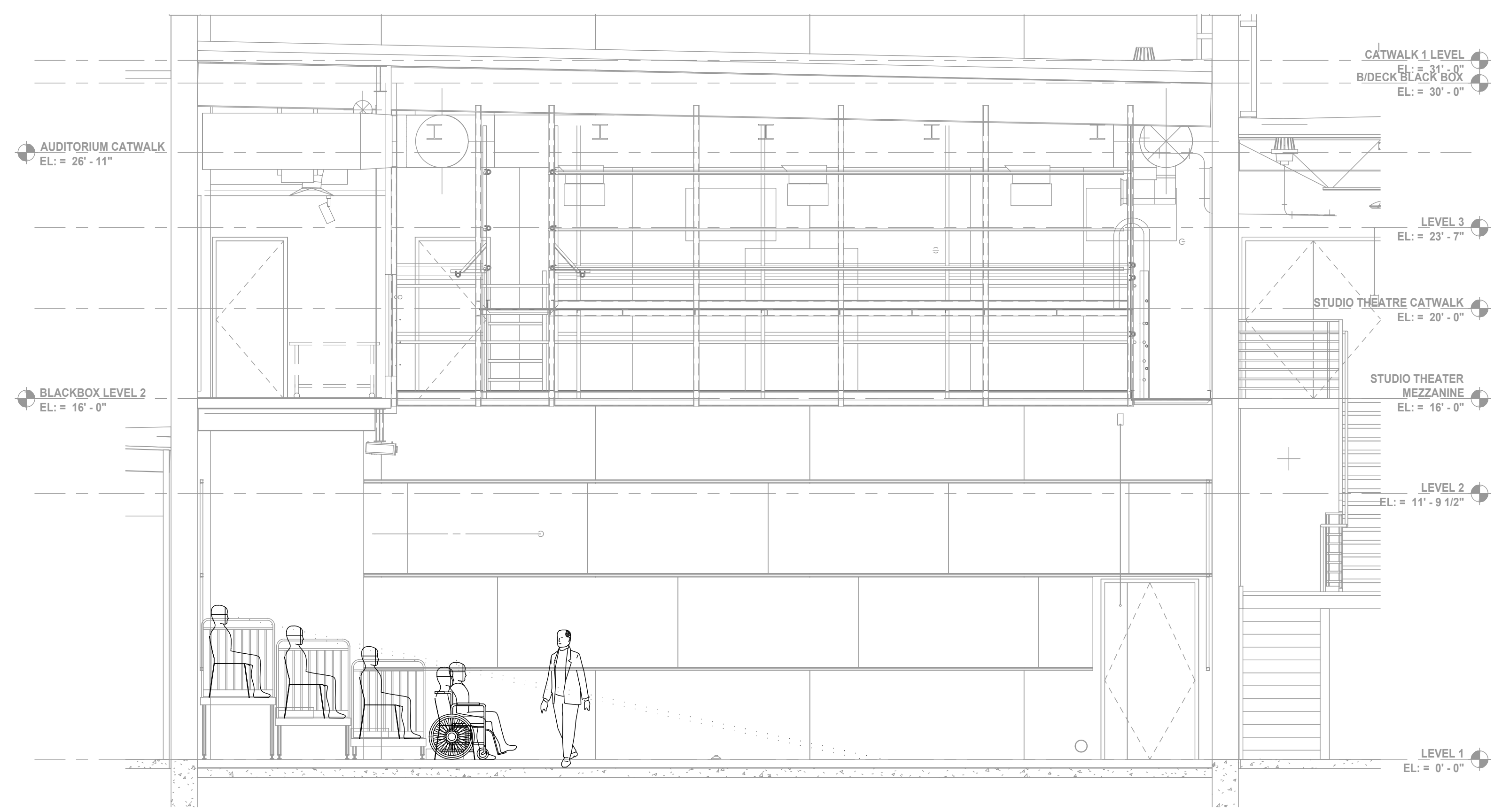
14 SECTION - THRUST SEATING LAYOUT B SCALE: 1/4" = 1'-0"
