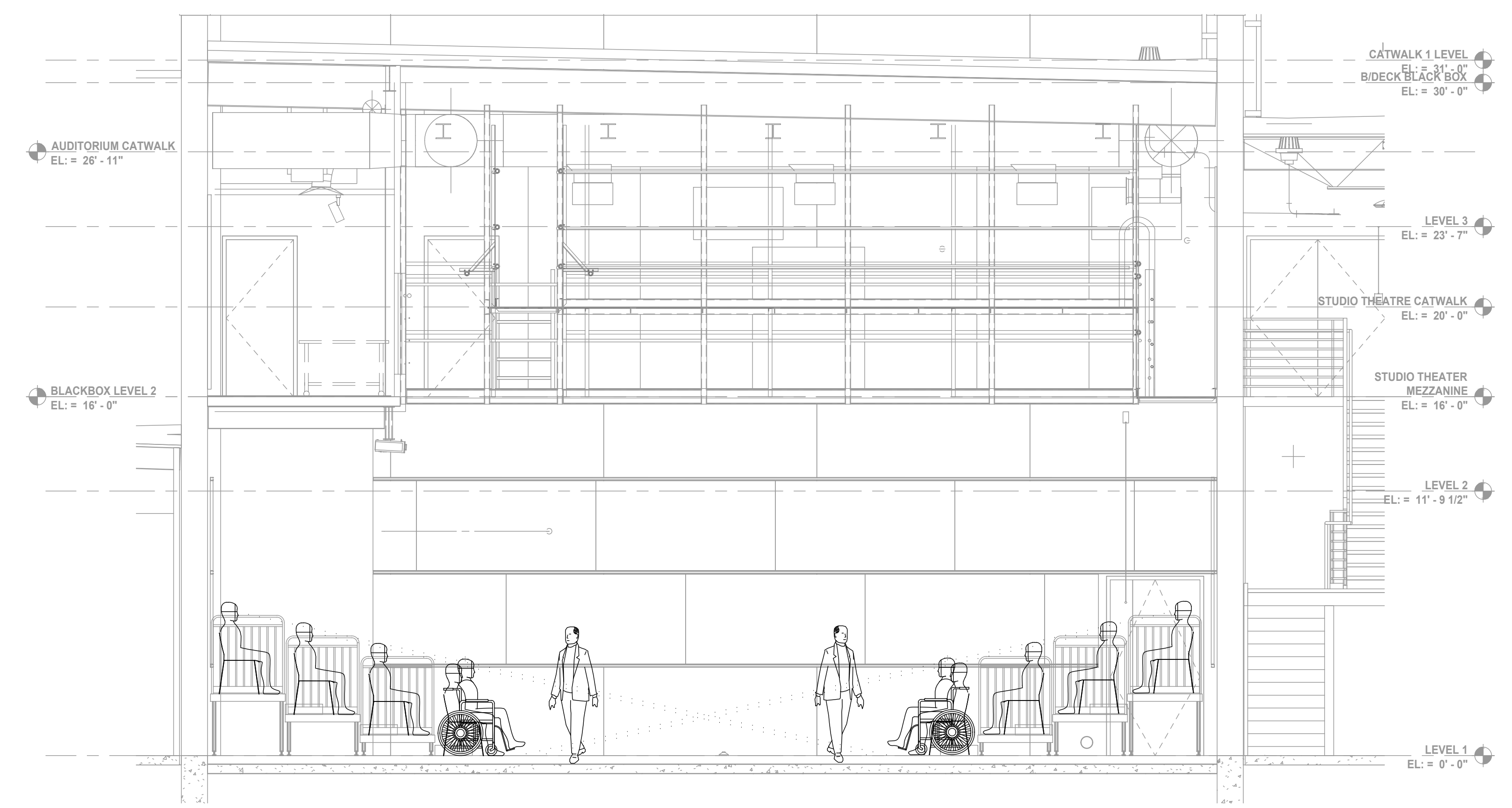
4 SECTION - THRUST SEATING LAYOUT A SCALE: 1/4" = 1'-0"
