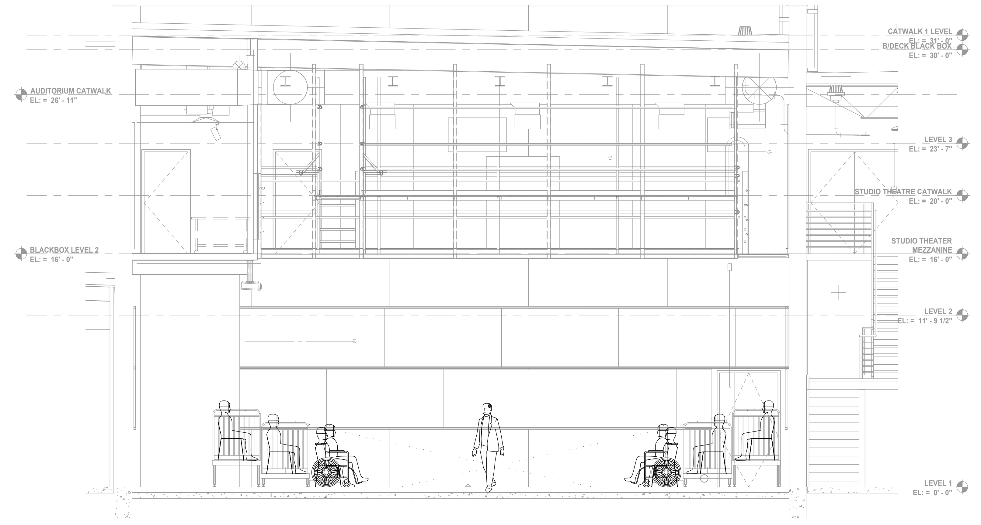
4 SECTION - ARENA SEATING LAYOUT SCALE: 1/4" = 1'-0"
