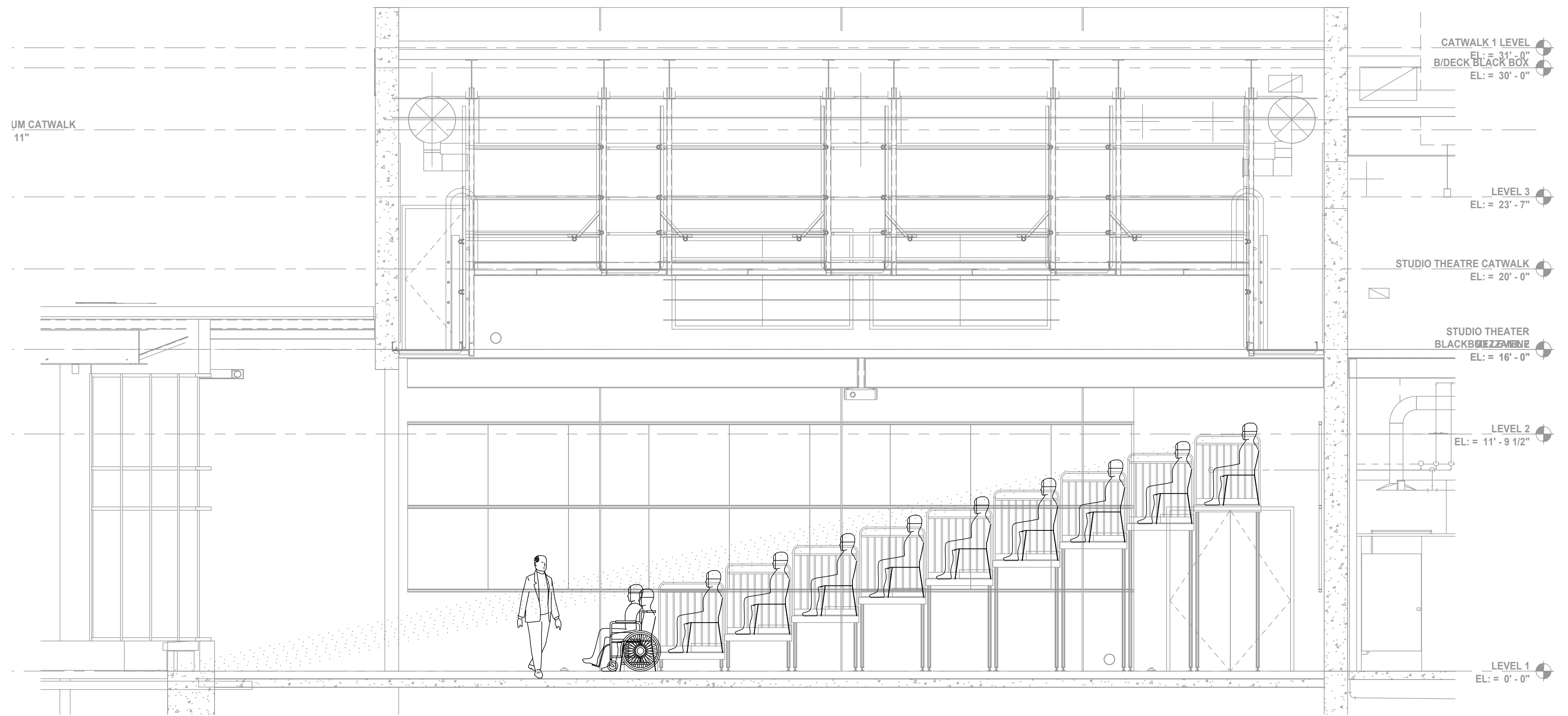
3 SECTION - END STAGE SEATING LAYOUT A SCALE: 1/4" = 1'-0"
