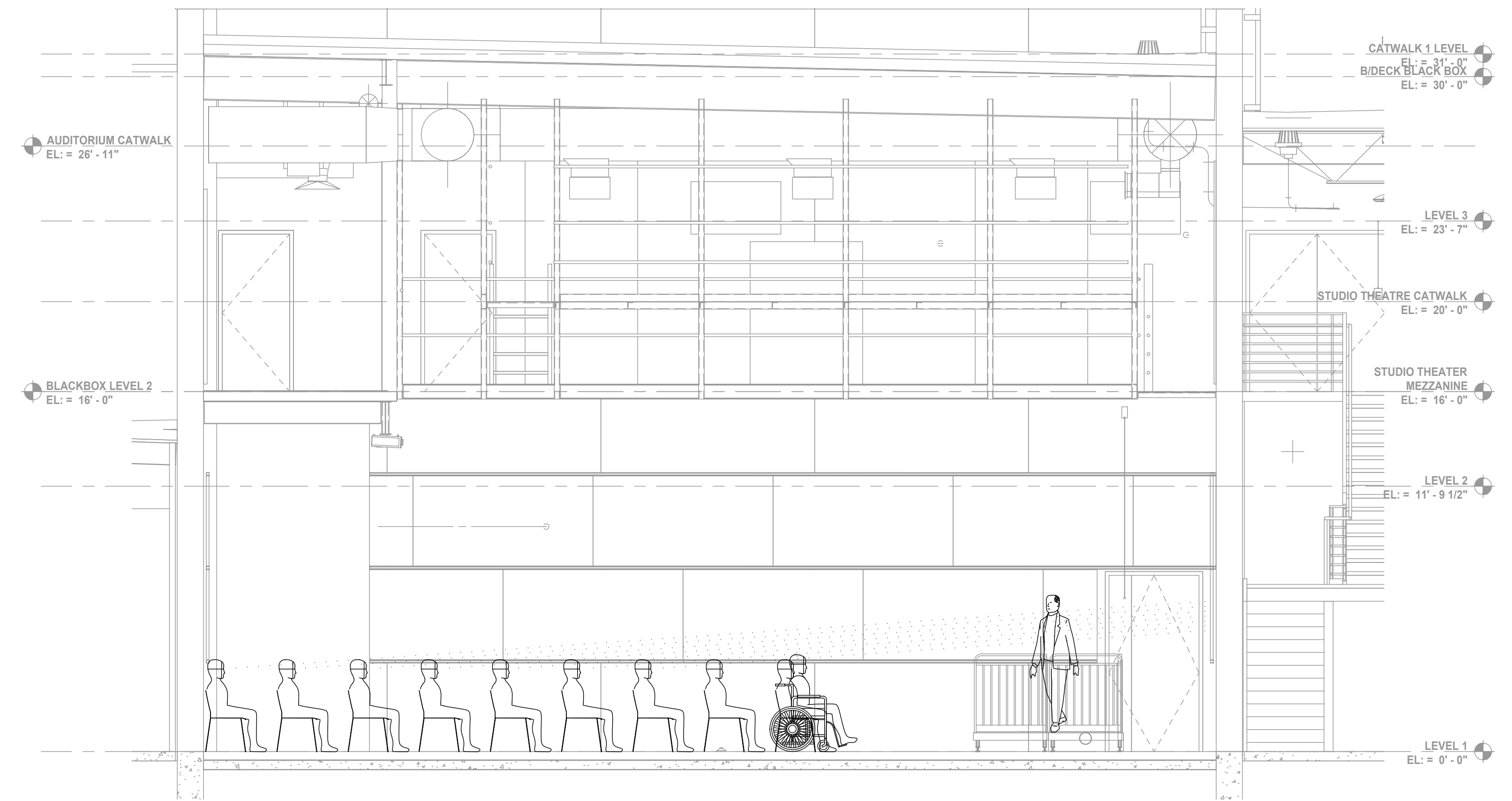
3 SECTION - LECTURE SEATING LAYOUT SCALE: 1/4" = 1'-0"
