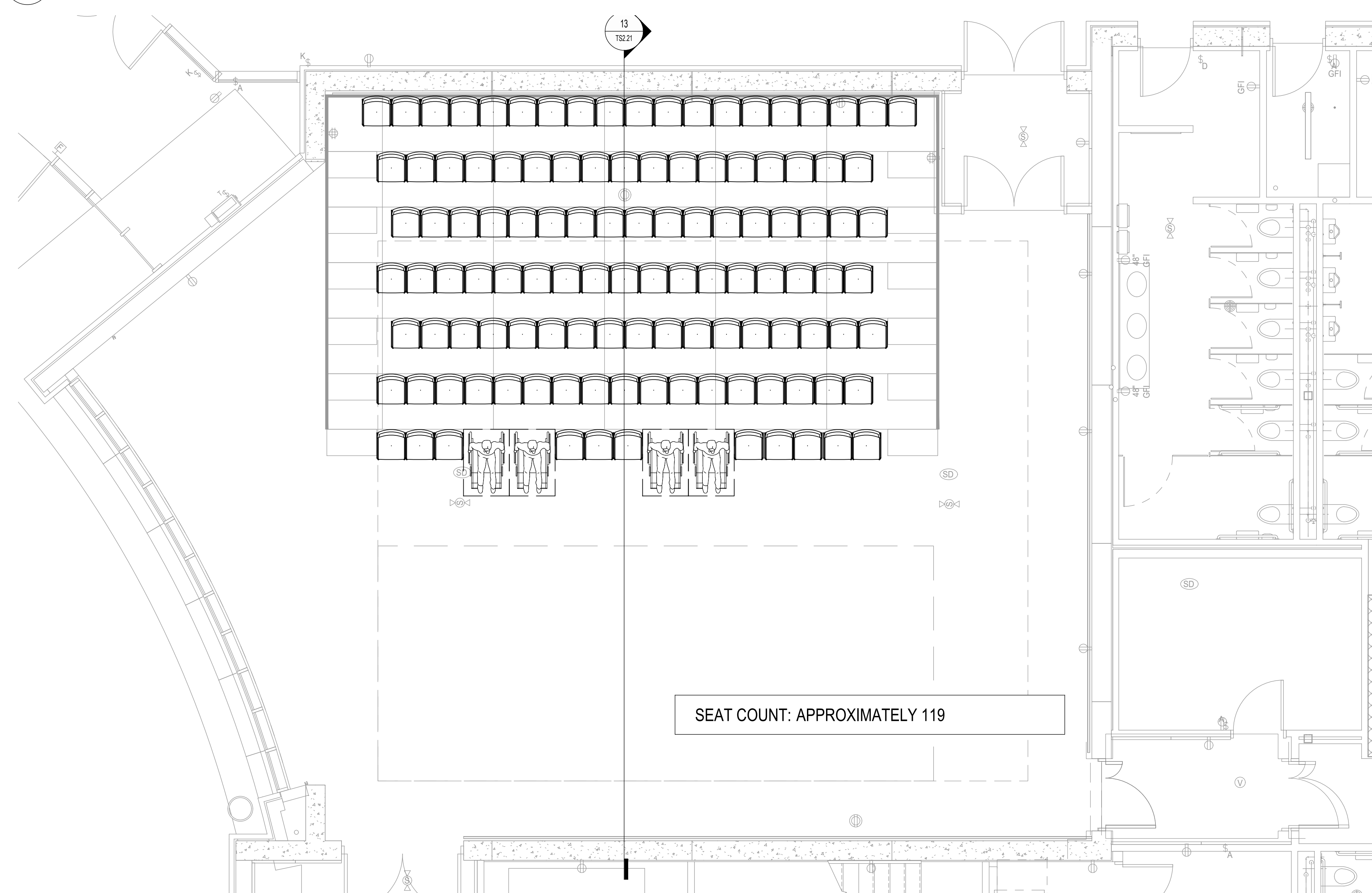
11 PLAN - END STAGE SEATING LAYOUT B SCALE: 1/4" = 1'-0"
